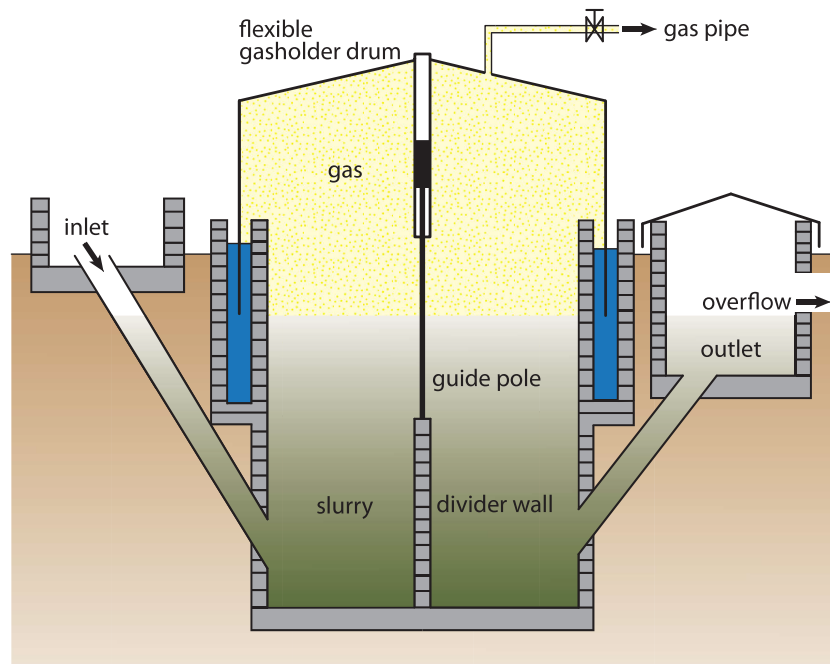
Figure 4: Floating-drum biogas plant (source: Vögeli, 2014)
