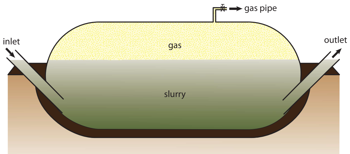
Figure 5: Tubular polybag digester (source: Vögeli, 2014)
